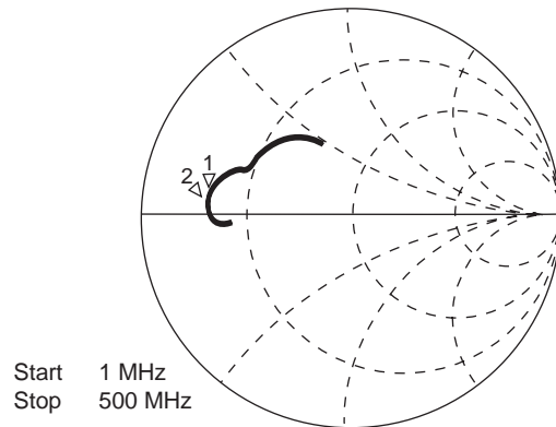
S22-FREQUENCY
